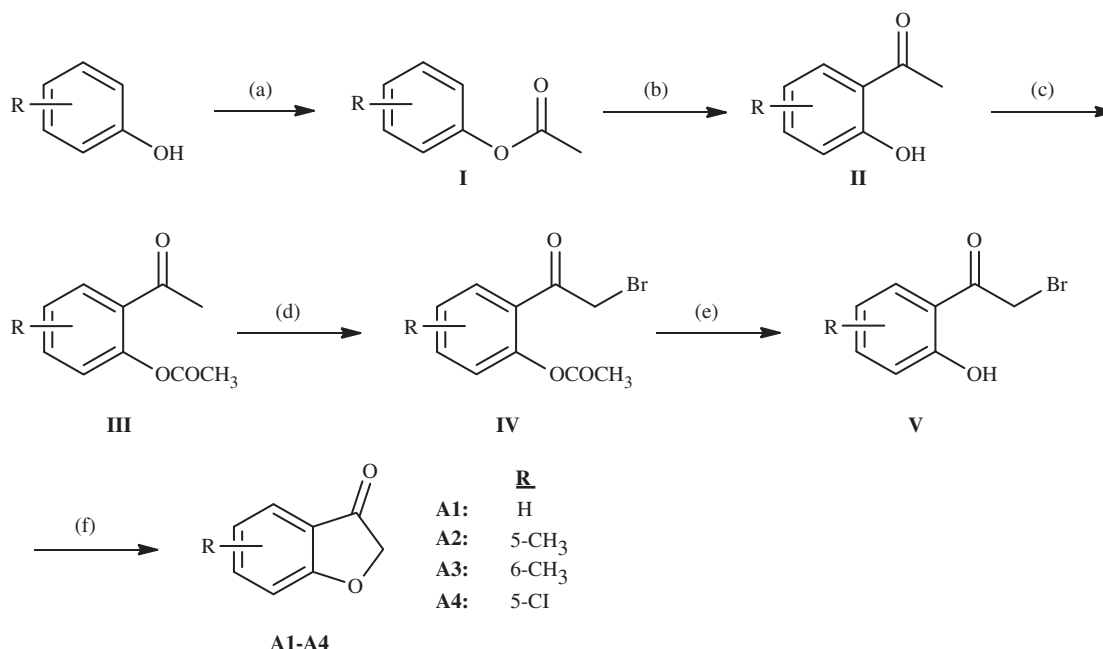
Scheme 1. The synthesis of the benzofuran-3-one derivatives ( A1–A4 ). Reactants/reagents and reaction conditions. a: (\text{CH}_3\text{CO})_2\text{O} , reflux, 30 min; b: \text{AlCl}_3 , 160–170 °C; c: (\text{CH}_3\text{CO})_2\text{O} , 50–100 °C, 3–4 h; d: \text{Br}_2 , \text{HBr} , diethyl ether or acetic acid; e: 10% HCl, reflux; f: \text{CH}_3\text{COONa} , EtOH, reflux.
