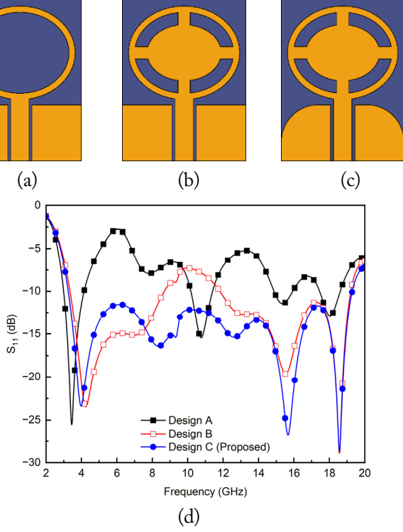
Fig. 2. Design evolution: (a) Design A, (b) Design B, (c) Design C, and (d) S_{11} of design evolution.
