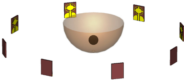
Fig. 10. Near-field microwave imaging setup with a tumor inside a breast phantom.
