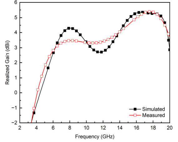
Fig. 7. Simulated and measured gain.
